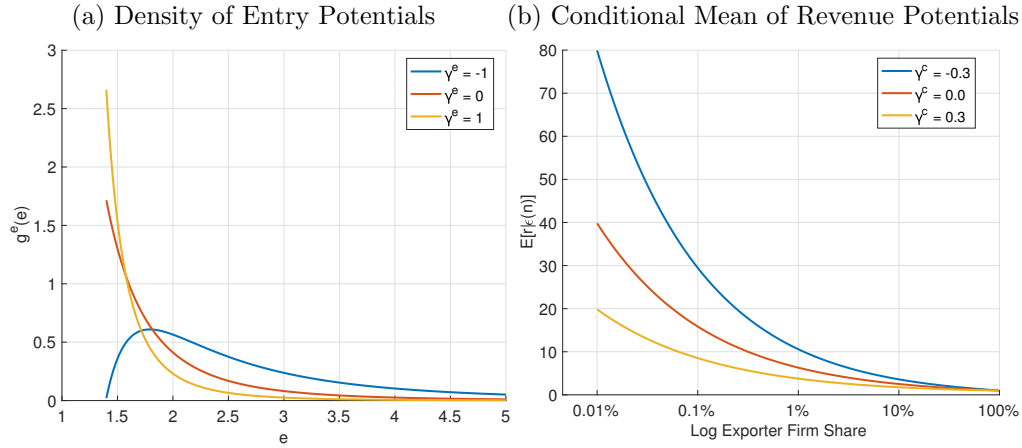
Figure OA.1: Distributional Assumptions and the Firm Export Margins
